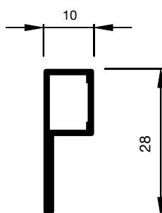
A1.3002 Rail P
