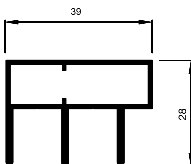
A1.3008 Rail W
