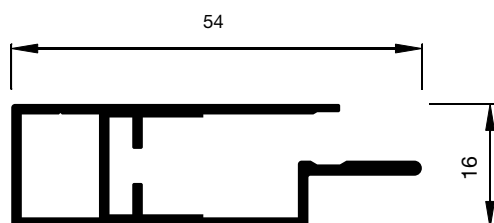
A1.3010 Softclose Schiene
