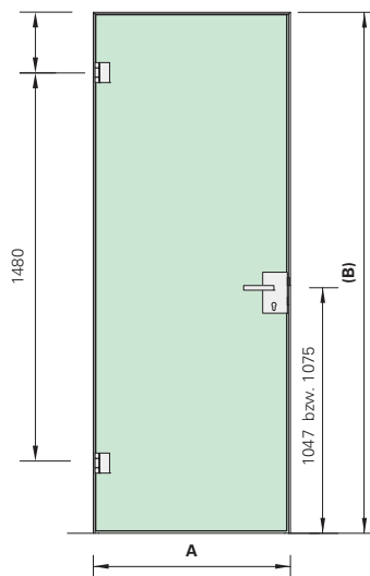
AT 23 - Anschlagtürzarge
