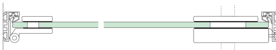
AT 23 – Dorma Spezialband, Juniorschloss (Office, Office Classic)
