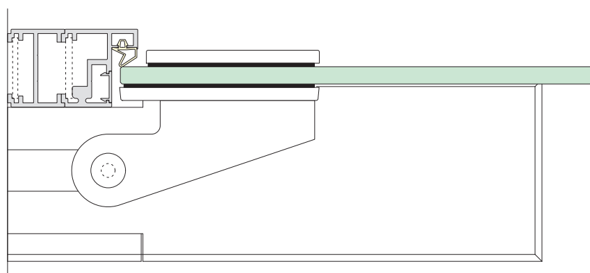
AT-44, Dorma EA-Program - Bodentürschliesser BTS 75
