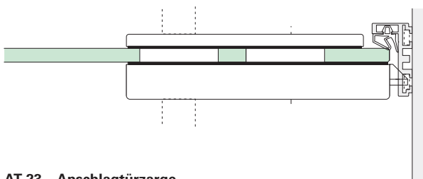
AT 23 – Anschlagtürzarge
